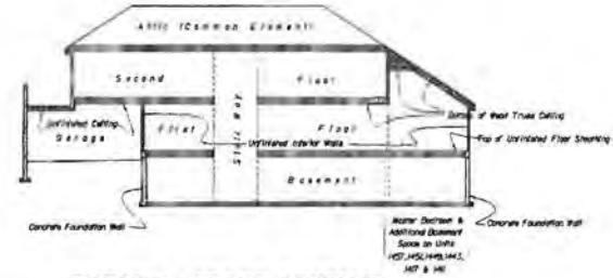
TYPICAL CROSS-SECTION Of Townhome Unit
