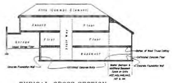
TYPICAL CROSS-SECTION Of Townhome Unit
